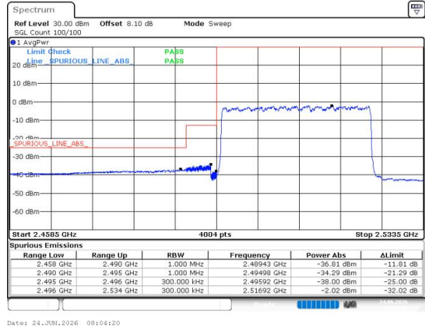
n41 SCS=30kHz DFT_QPSK BW=30MHz LowChannel=502200 RB=75@0
