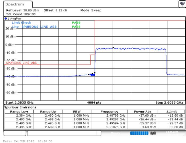
n41 SCS=30kHz DFT_64QAM BW=90MHz LowChannel=508200 RB=243@0
