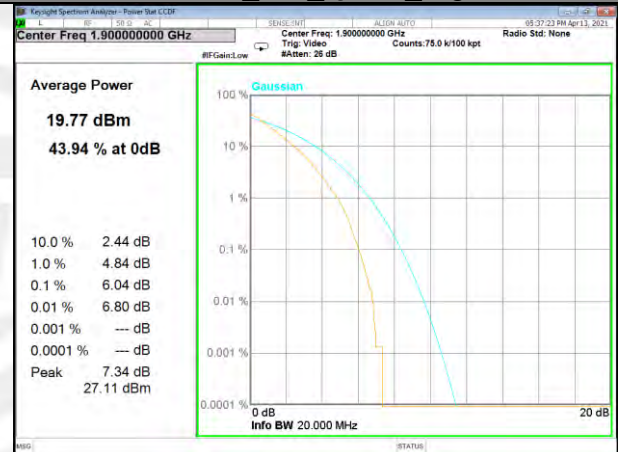
Band 2_100_Q16_High
