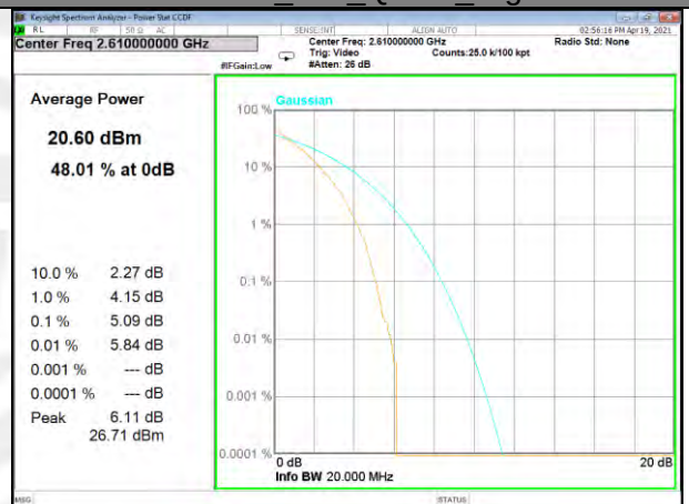
Band 38_100_Q16_High
