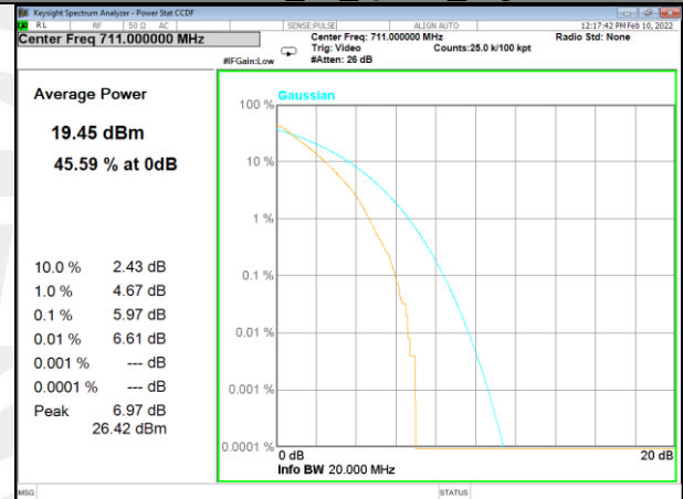
Band 12_50_Q16_High
