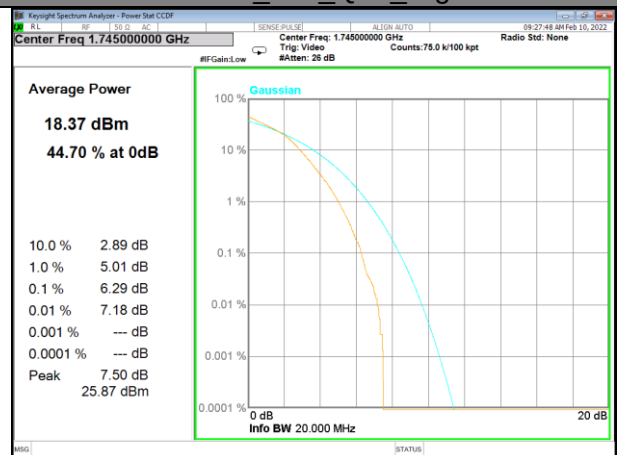
Band 4_100_Q16_High
