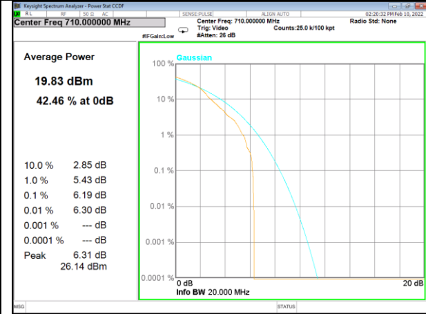
Band 17_1_QPSK_High
