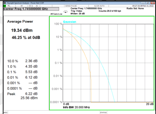
Band 4_100_Q16_High
