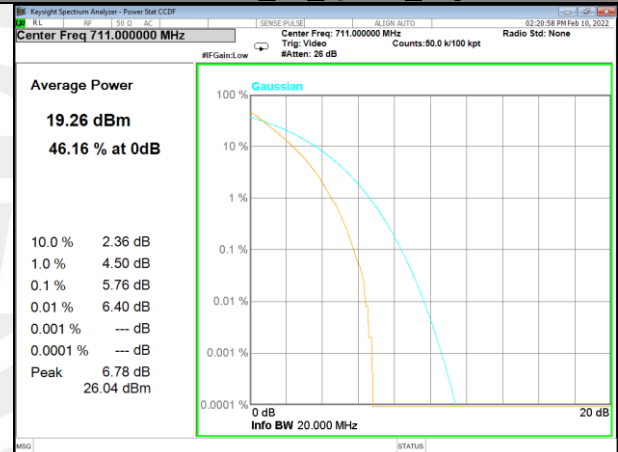
Band 17_50_Q16_High
