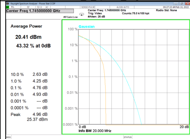
Band 4_1_Q16_High
