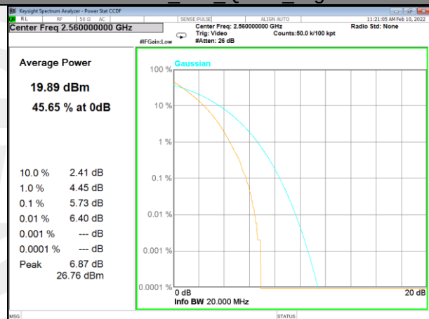
Band 7_100_Q16_High
