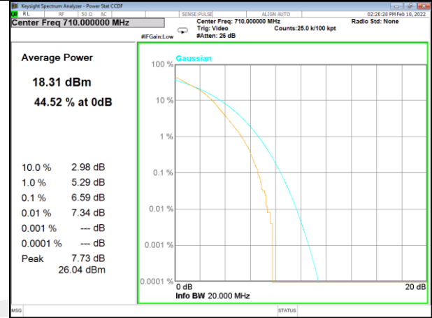
Band 17_50_QPSK_High
