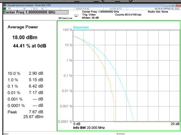
Band 2_100_Q16_High
