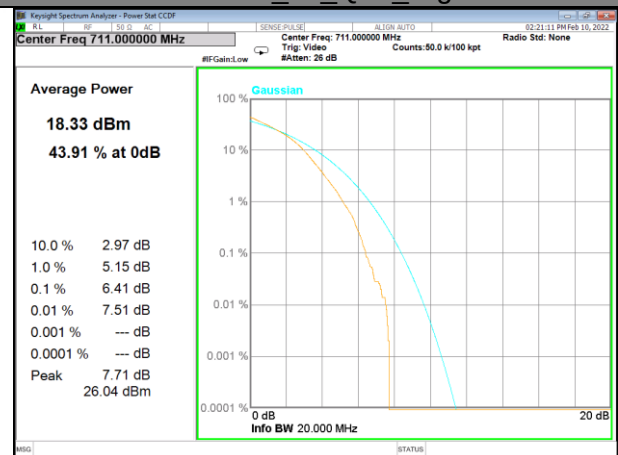
Band 17_50_Q16_High
