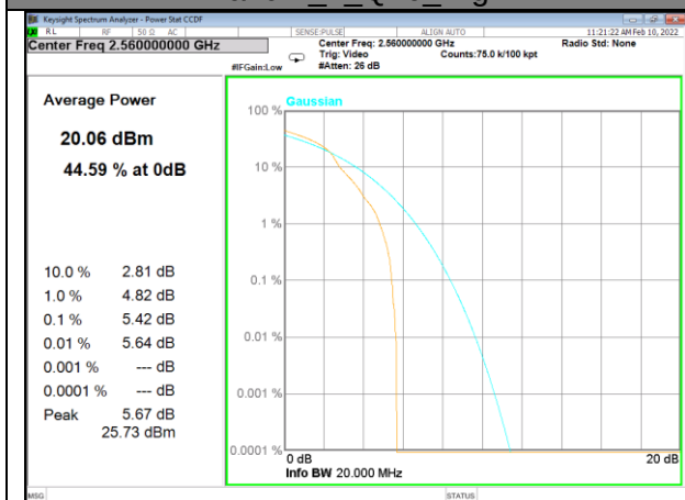
Band 7_1_Q16_High
