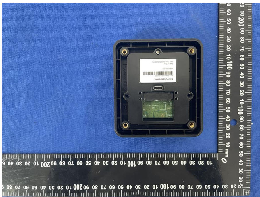
REAR VIEW OF EUT VPOS M S-CLS(Machine head: Black)
