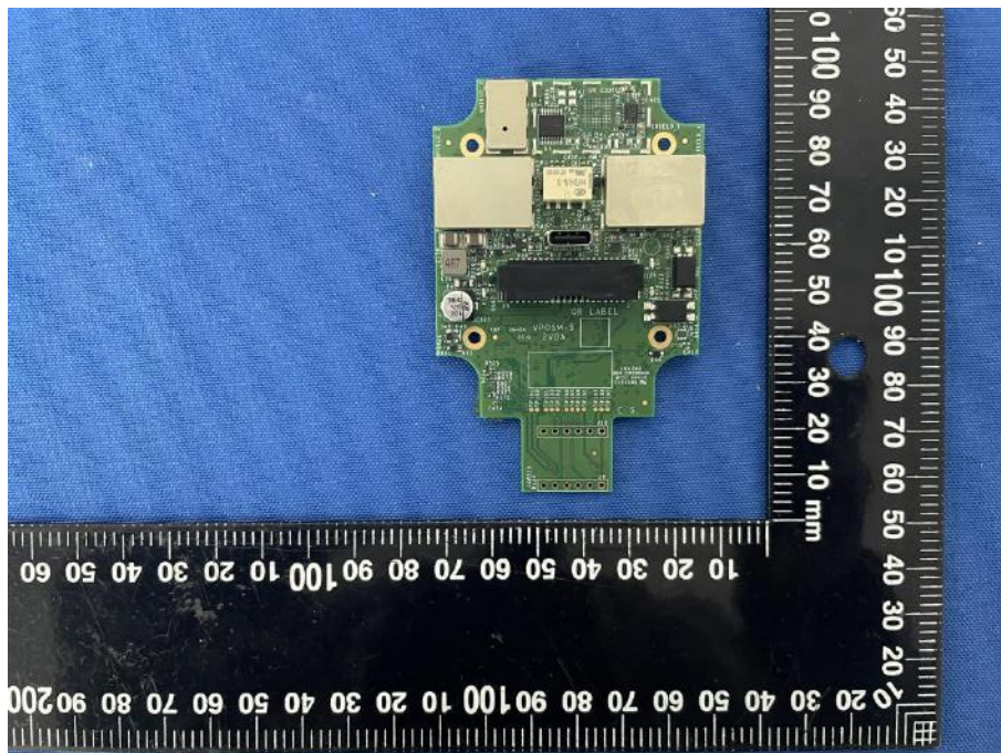
SECONDARY BOARD 1 TOP VIEW (WITH SHIELDING)
