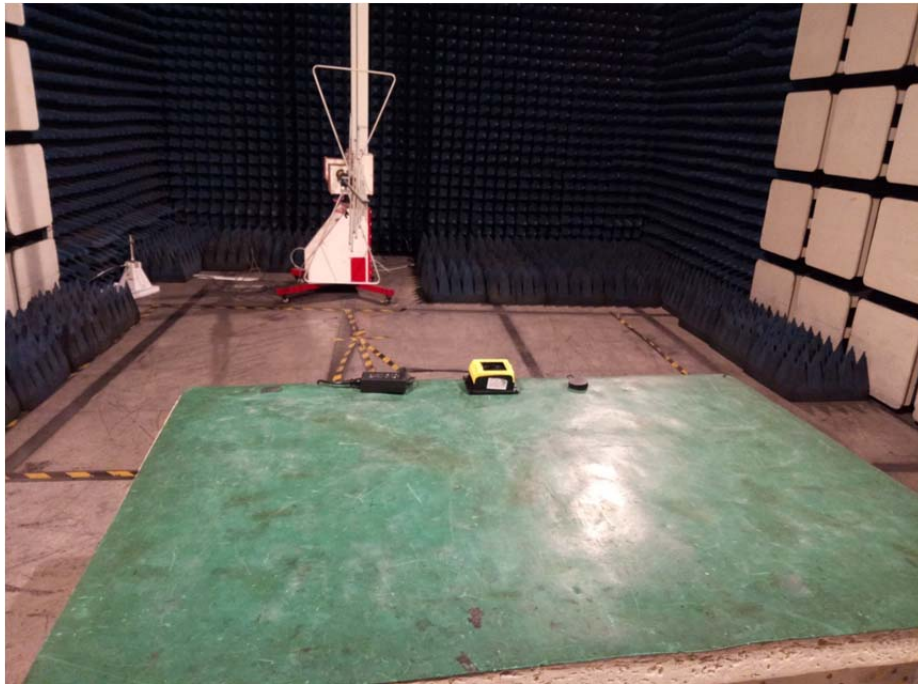
Radiation Emission
