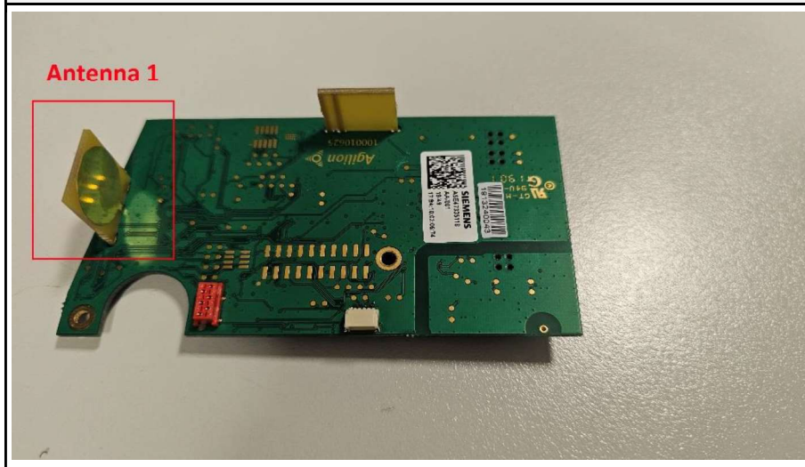
Antenna 1 - Left
