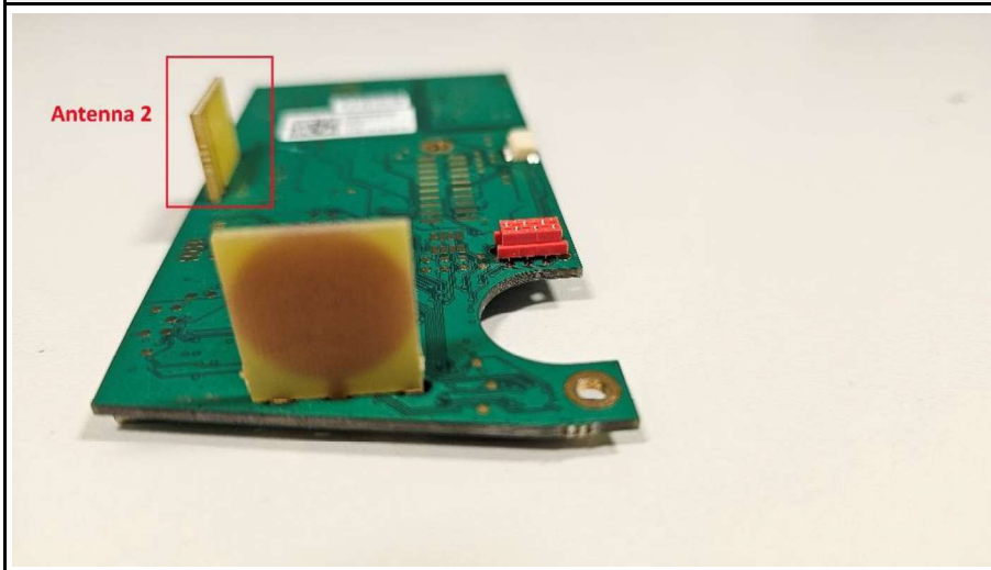
Antenna 2 - Right
