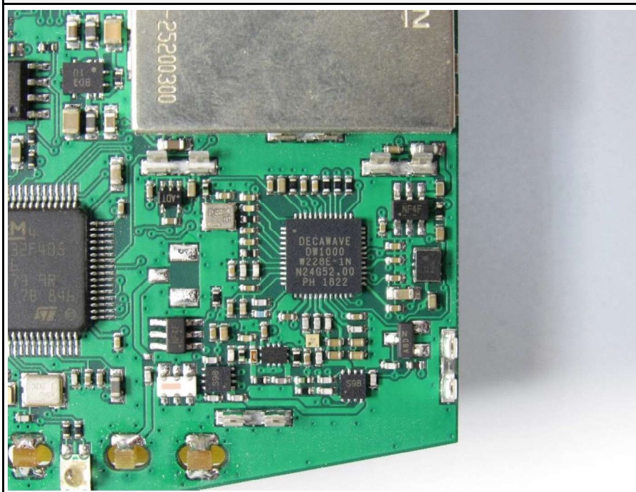
Radio part
