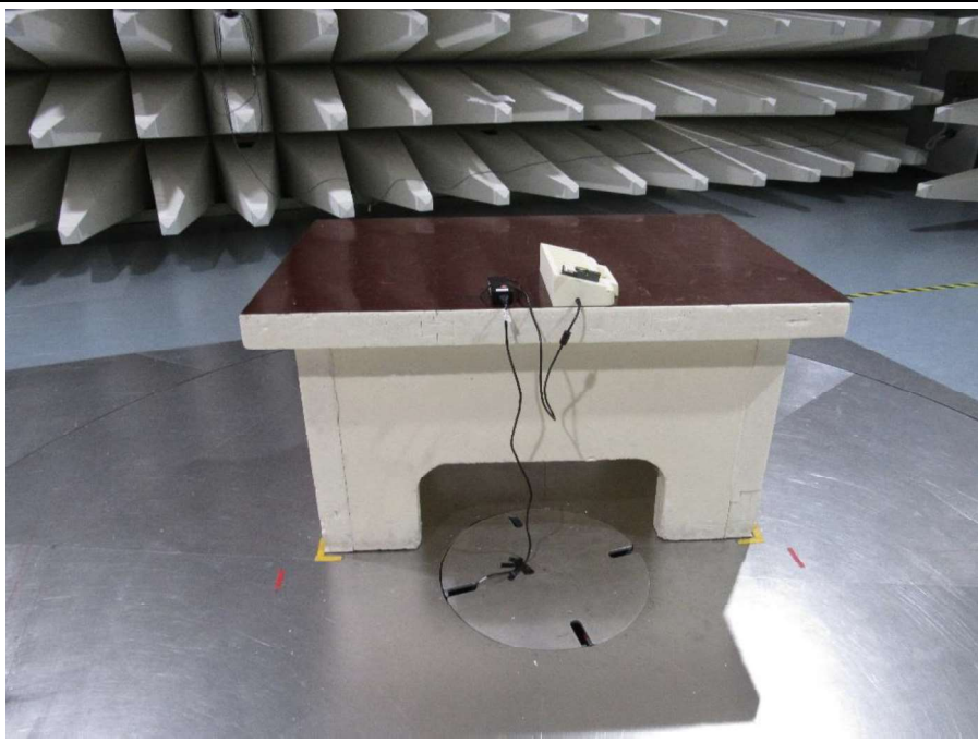
EUT SETUP FOCUS CONFIGURATION 2 AC6
