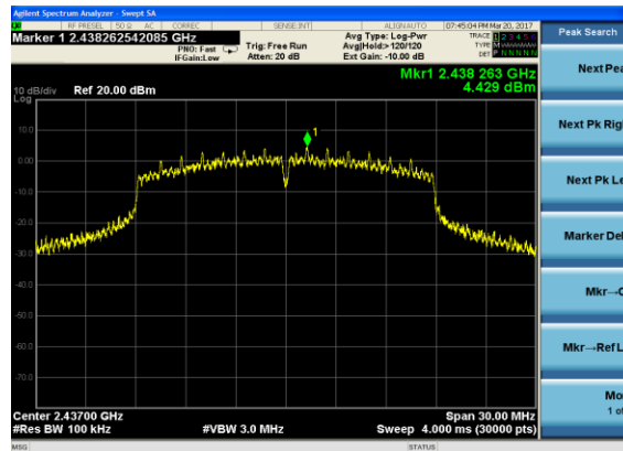
Ant. Port 1
