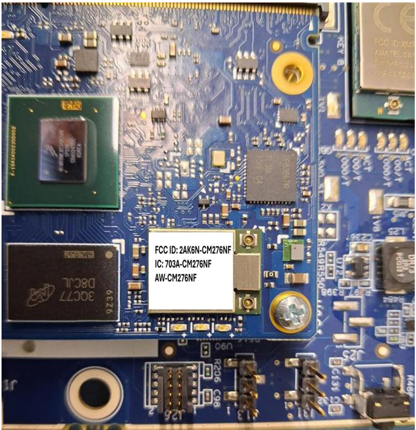
AW-CM276NF Wi-Fi and BT Module – External Photo with new UTEC Label
