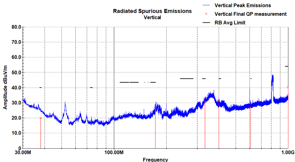
Vertical Plot – 30-1000MHz – Mid Channel
