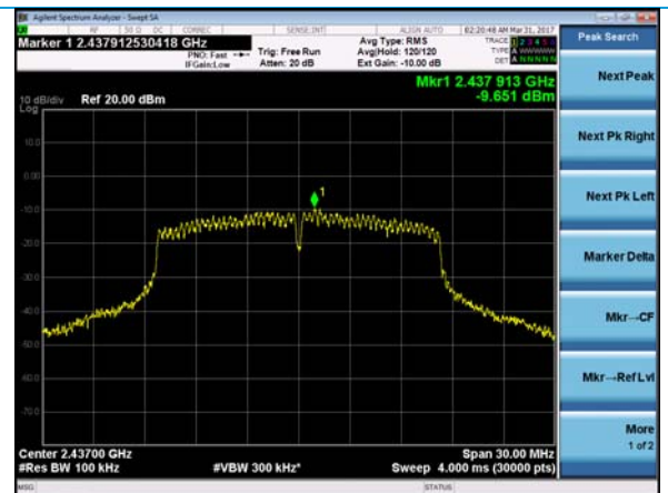
54 Mbps – Mid Channel
