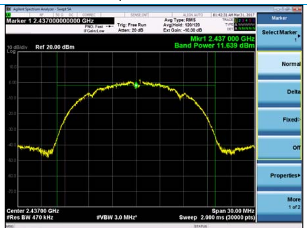
11 Mbps – Mid Channel
