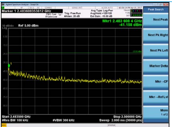
MCS0 – Upper Band Edge – Channel 11
