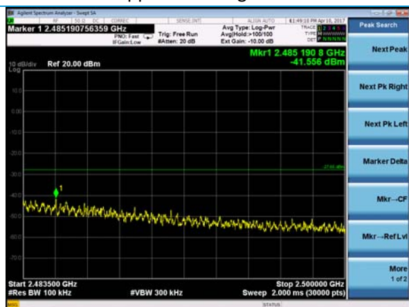
MCS7 – Upper Band Edge – Channel 11
