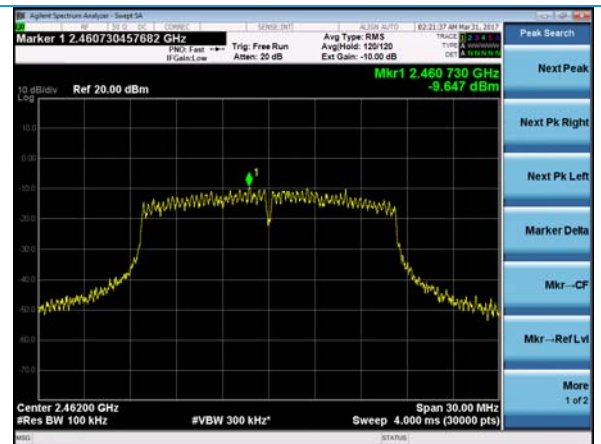
54 Mbps – High Channel
