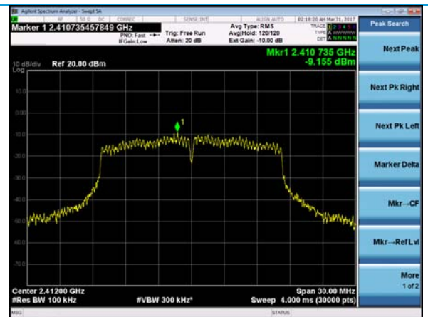
54 Mbps – Low Channel
