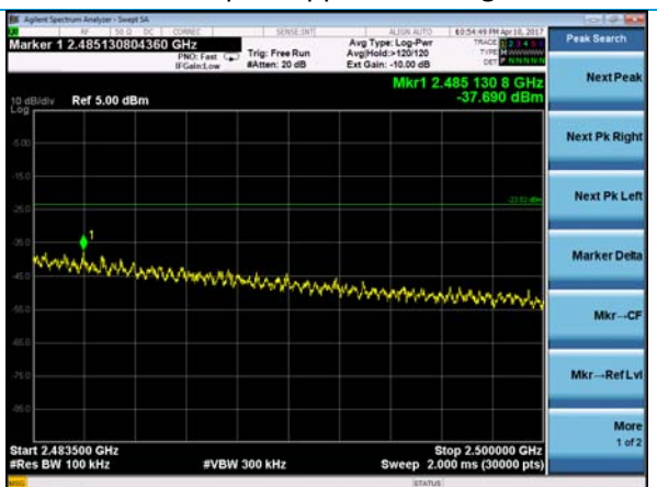
MCS0 – Upper Band Edge – Channel 10
