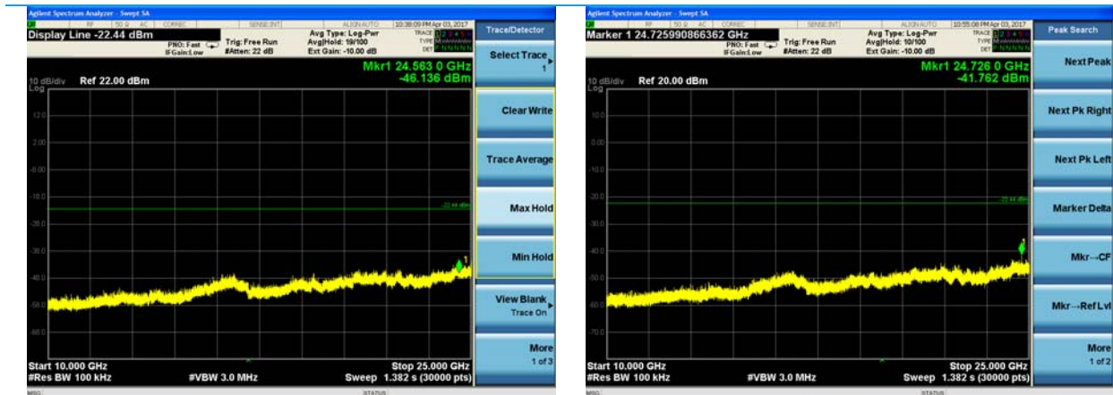
1 Mbps – High Channel – 10-25 GHz
