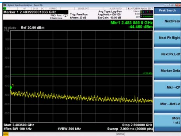
MCS7 – Upper Band Edge – Channel 10
