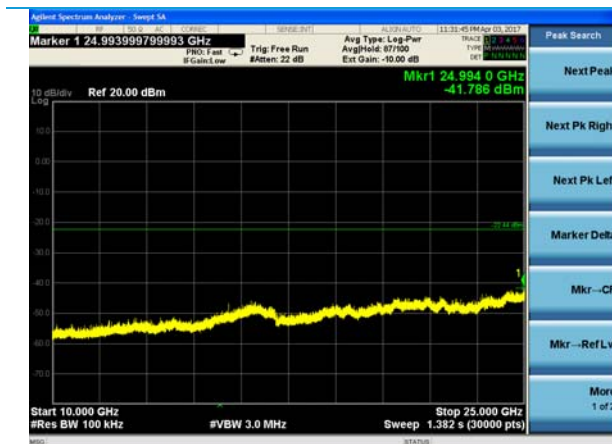
MCS7 – Low Channel – 10-25 GHz
