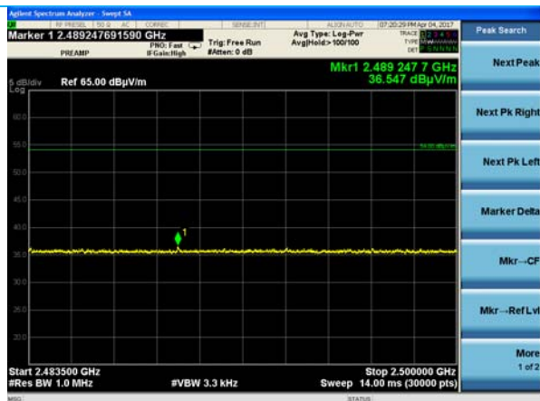
Upper Band-Edge – Channel 10 – Average
