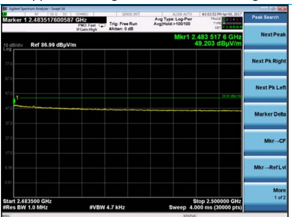
Upper Band-Edge – Channel 11 - Average
