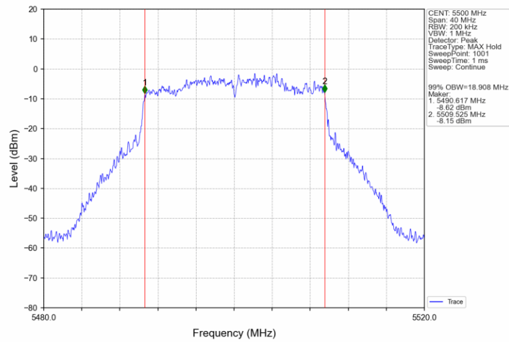
802.11ax(HEW20)_LCH_5500MHz_SU_/_Ant1_NTNV
