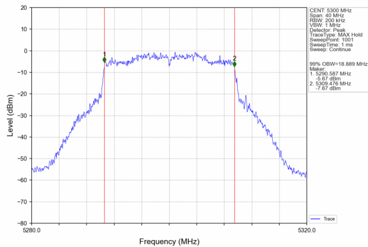
802.11ax(HEW20)_MCH_5300MHz_SU_/_Ant1_NTNV
