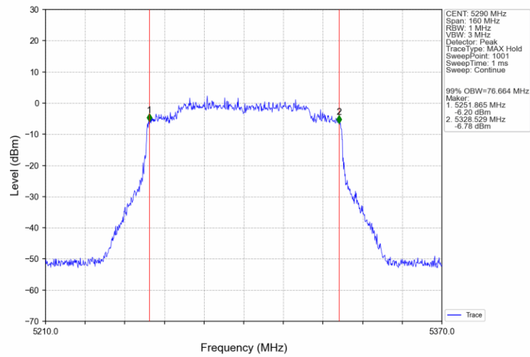
802.11ax(HEW80)_MCH_5290MHz_SU_/_Ant1_NTNV
