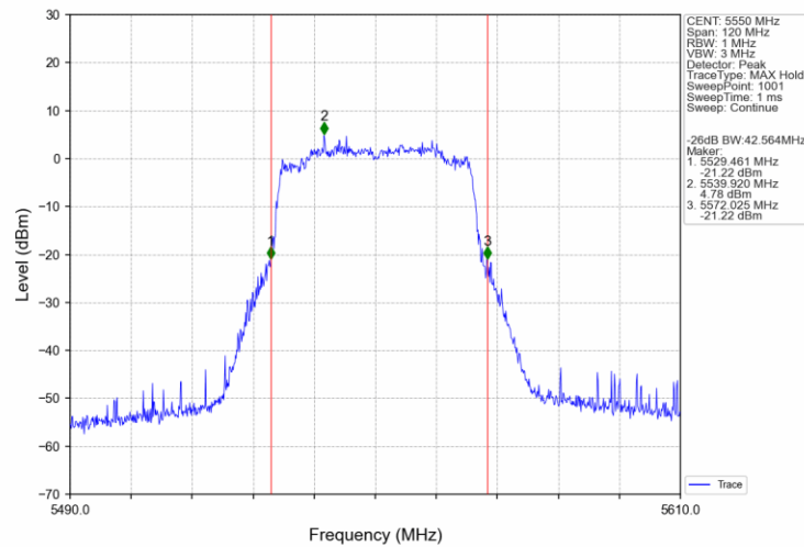
802.11ax(HEW40)_MCH_5550MHz_SU_/_Ant1_NTNV
