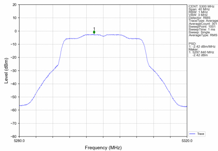
802.11ax(HEW20)_MCH_5300MHz_SU_/_Ant1_NTNV
