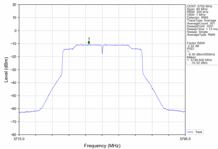
802.11ax(HEW40)_LCH_5755MHz_SU_/_Ant1_NTNV
