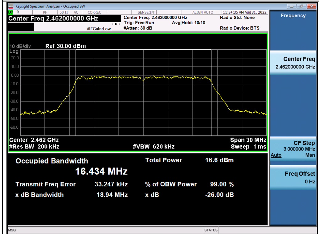
Test_Graph_802.11g_ANT3_2462_6Mbps_OBW
