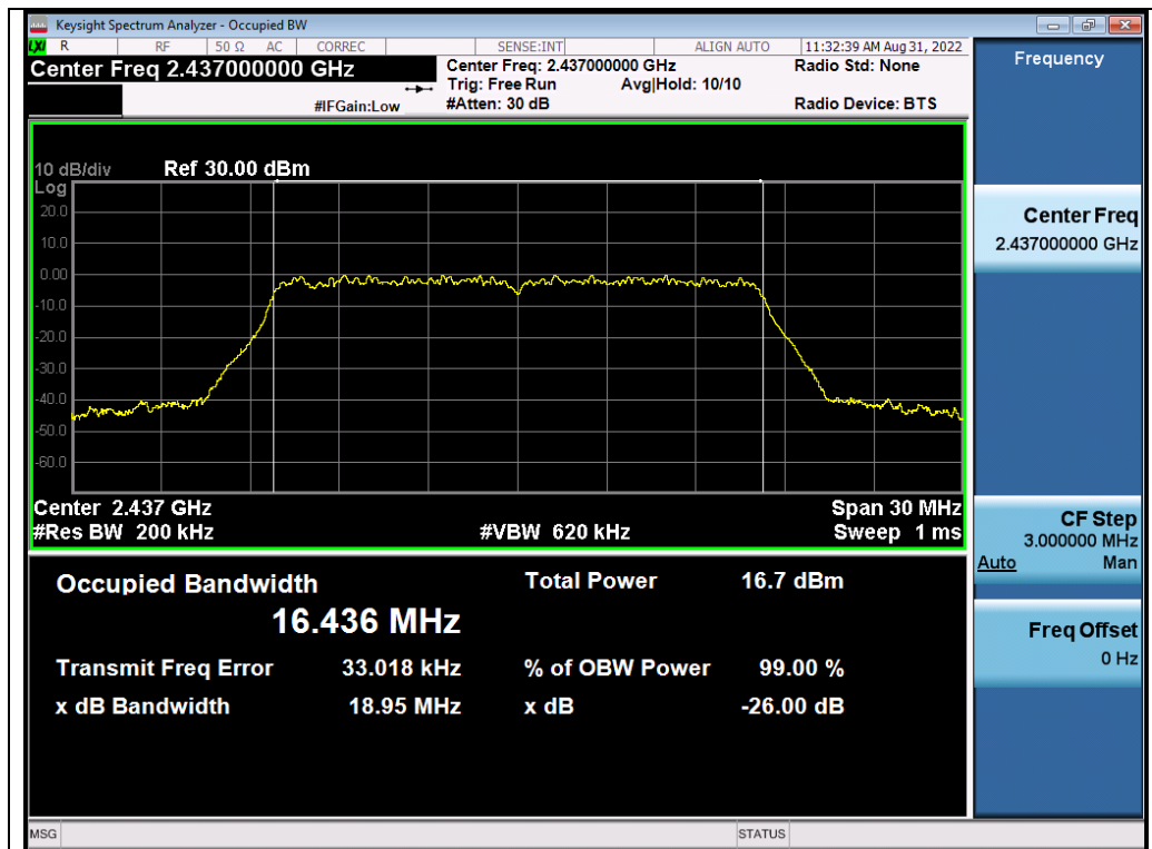
Test_Graph_802.11g_ANT3_2437_6Mbps_OBW
