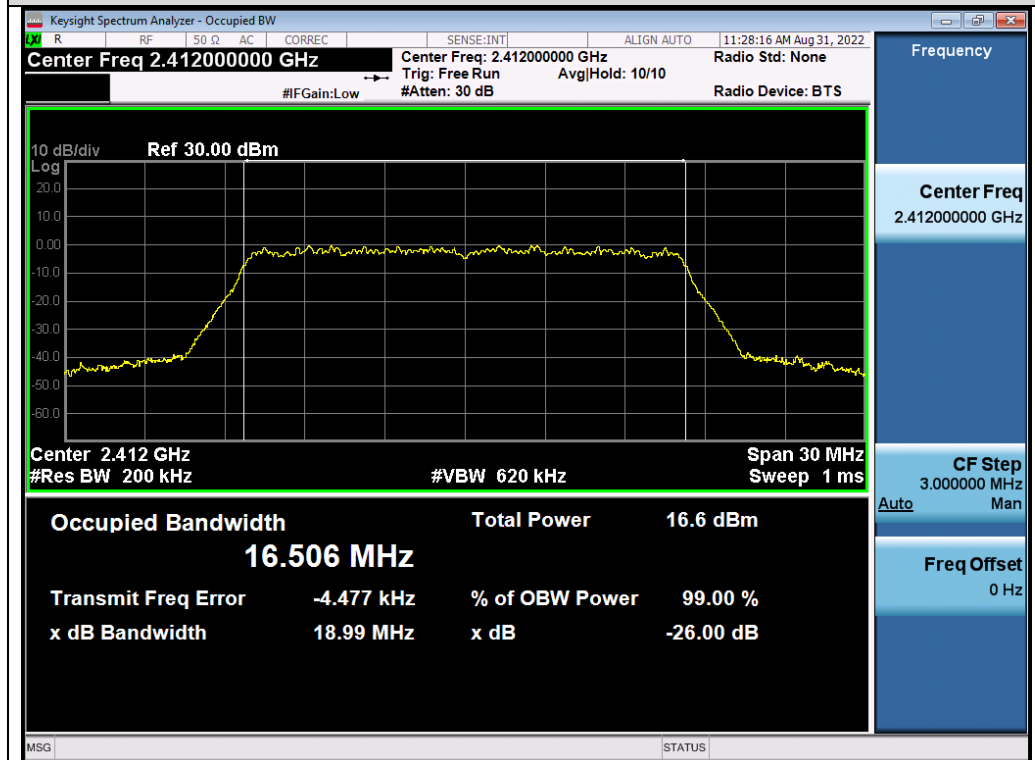
Test_Graph_802.11g_ANT3_2412_6Mbps_OBW
