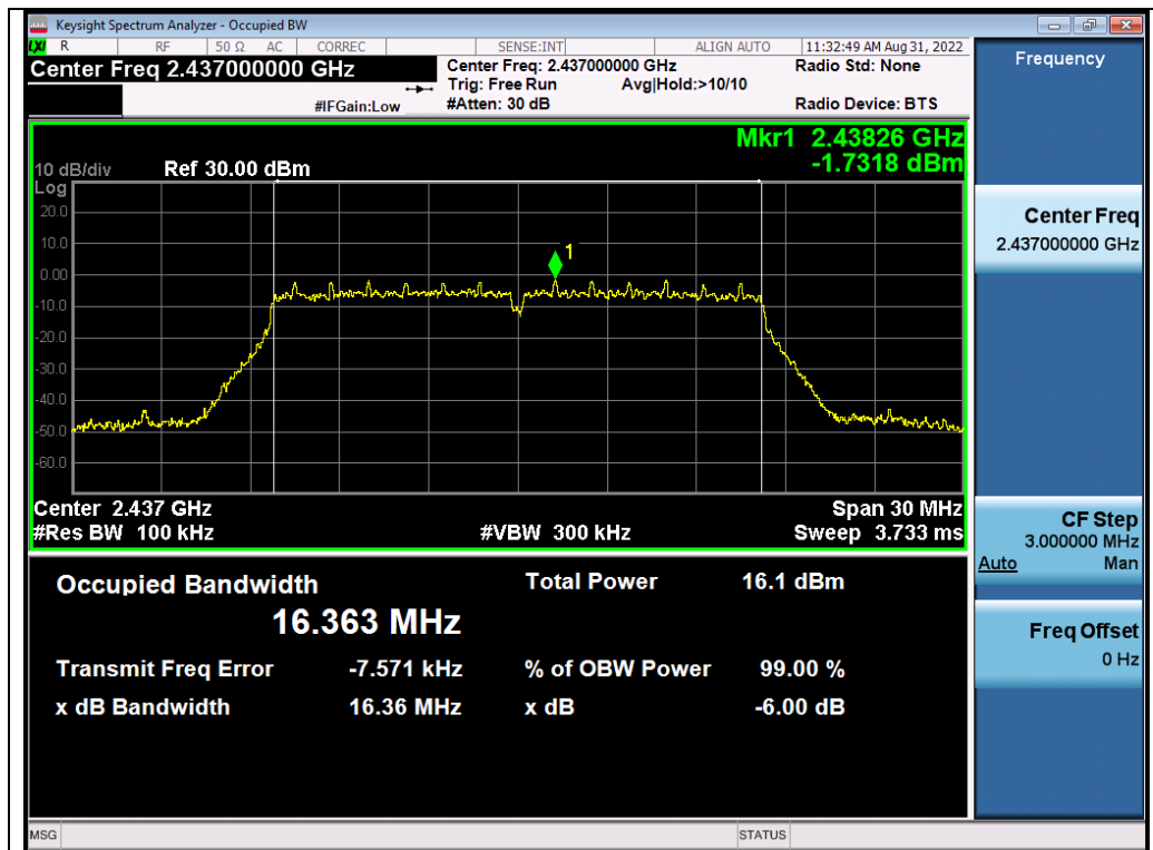
Test_Graph_802.11g_ANT3_2437_6Mbps_DTSBW
