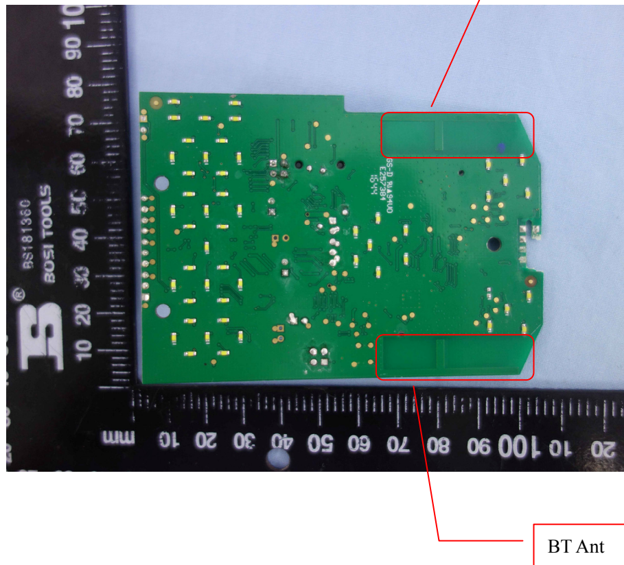
Solder Board-Component View 3
