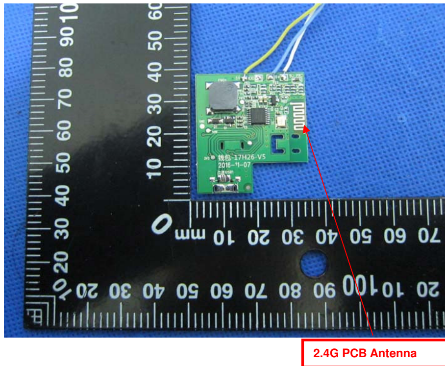
Photo 9 Appearance of PCB
