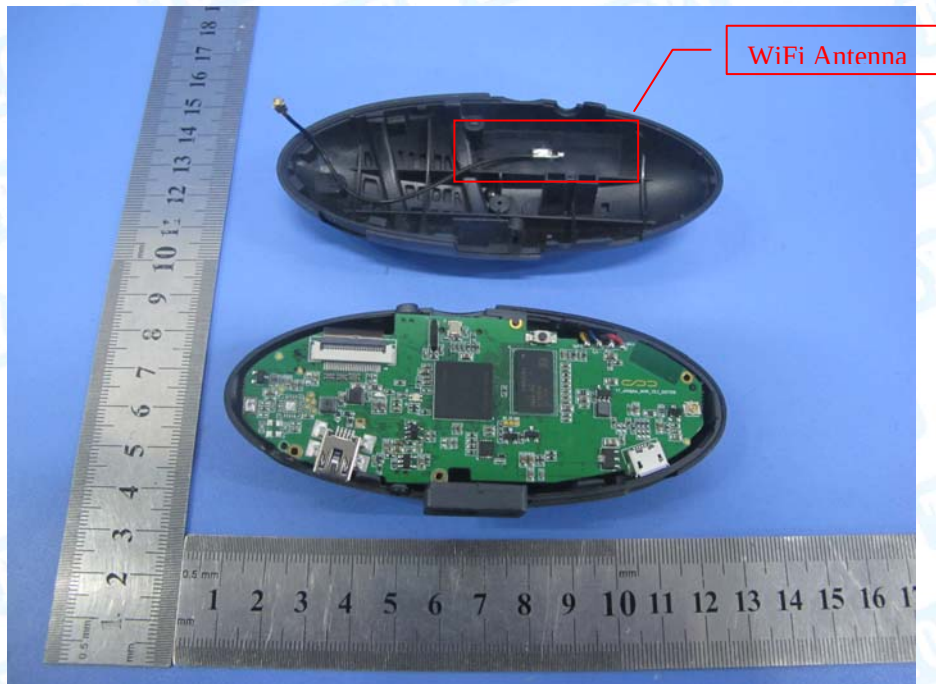
Photo 9 Internal of EUT
