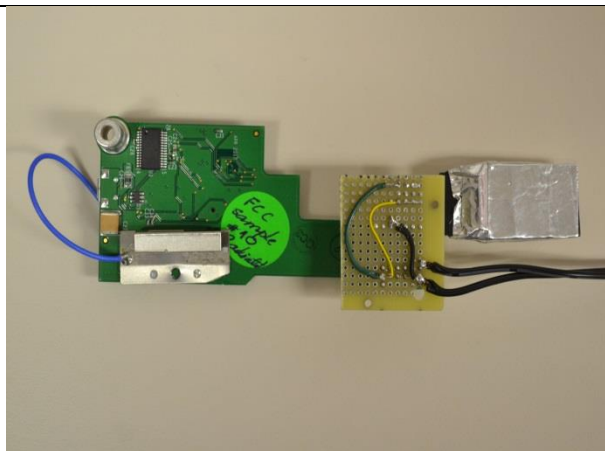
ANTENNA AT X POSITION FRONT PHOTO
