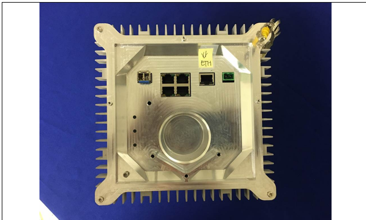
EUT I/O View
