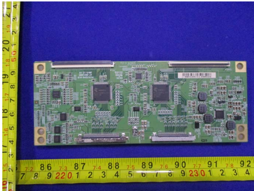
EUT – Mainboard of Display Screen Top View
