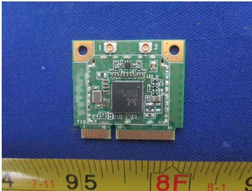
EUT – RF PCB Top Unshielded View
