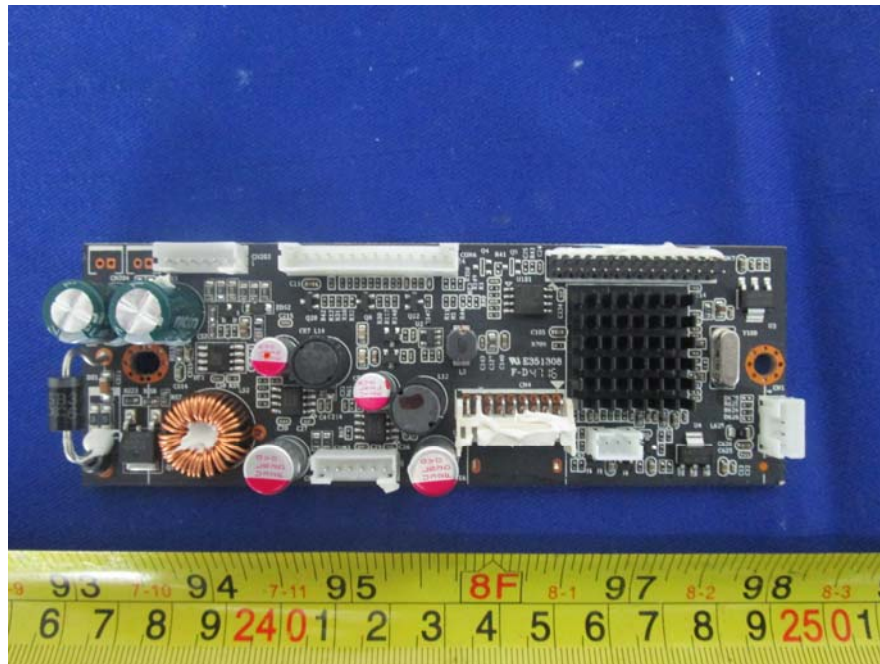
EUT –TSUM Board Top View
