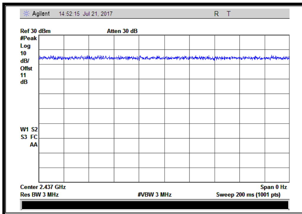
(Plot for Duty cycle, Channel 6: 2437MHz @ 802.11n-20)
