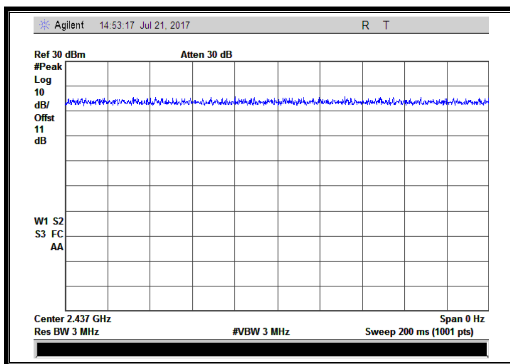
(Plot for Duty cycle, Channel 6: 2437MHz @ 802.11g)
