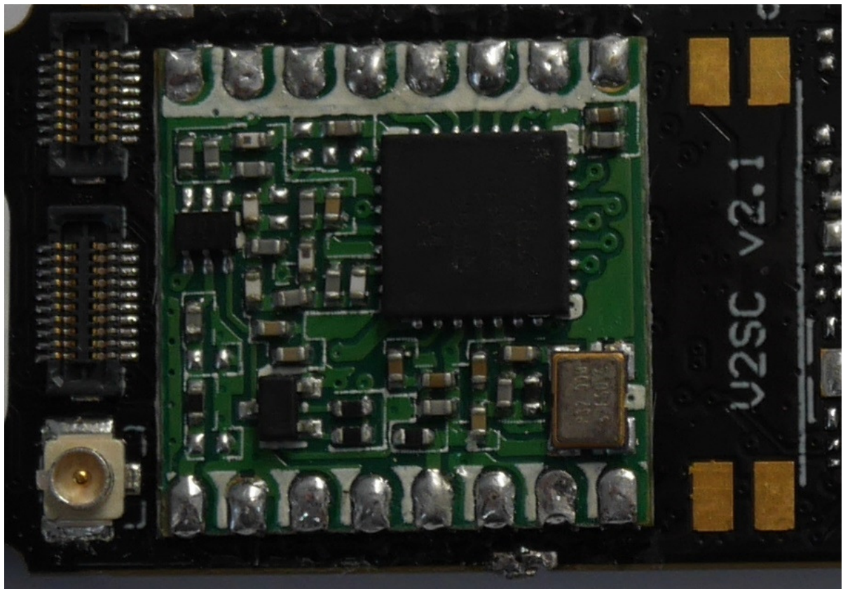
Radio Board
