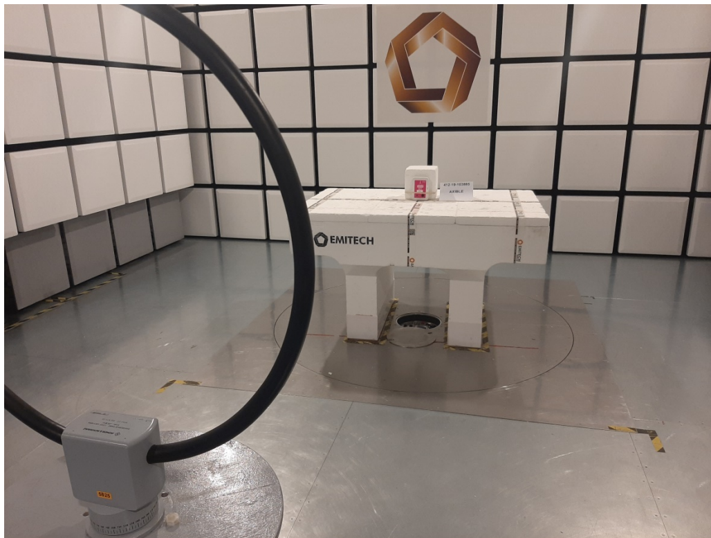
TEST SETUP PHOTO(S) RADIATED EMISSIONS (9KHz-30MHz)
