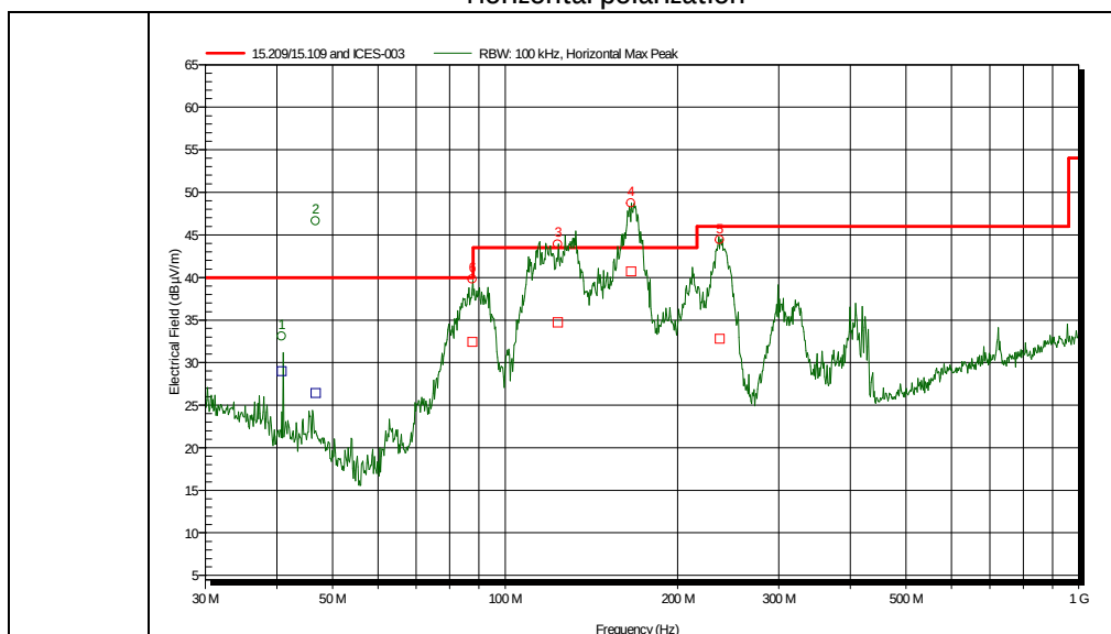
Horizontal polarization
