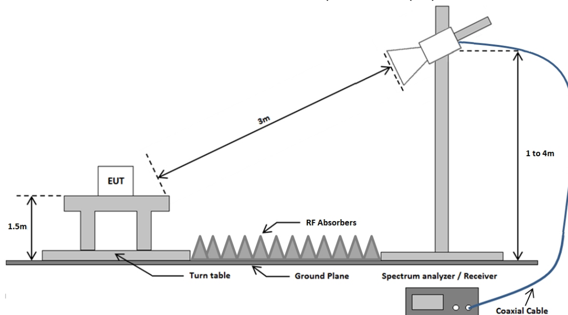
Radiated emissions test setup above 1 GHz (FCC)
