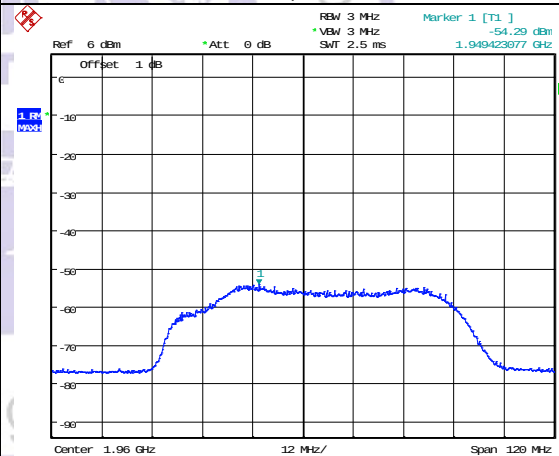
Downlink, 1930-1990MHz
