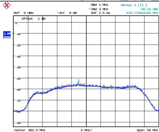
Downlink, 869-894MHz
