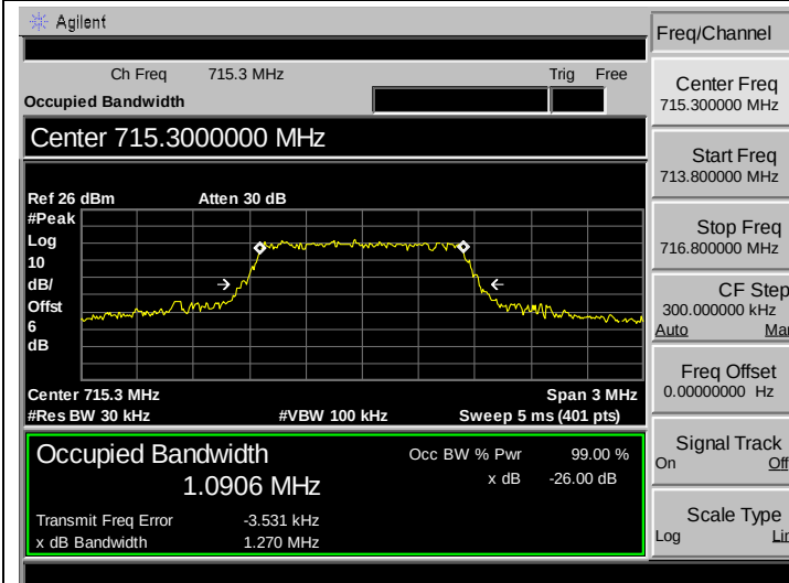
LTE BAND 12 (1.4MHz QPSK-High CH)
