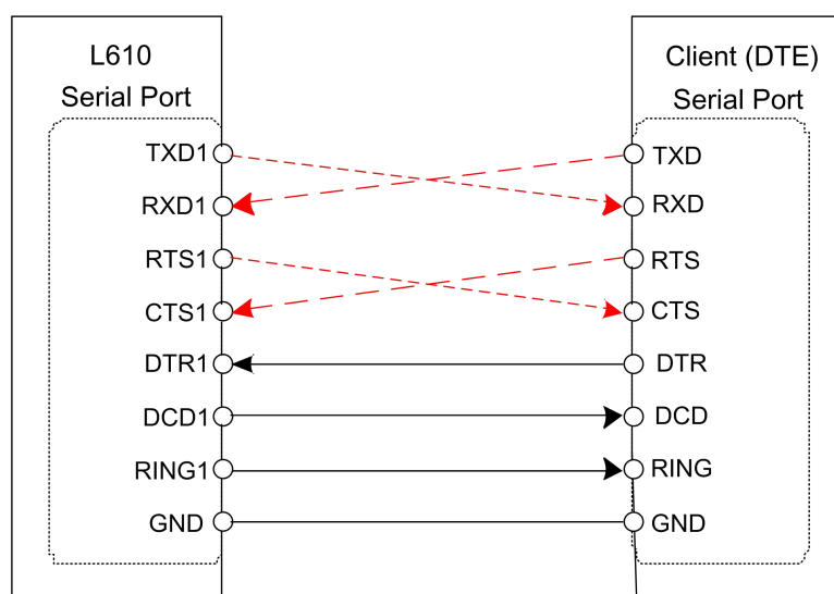
Figure 3-13 UART Full mode
