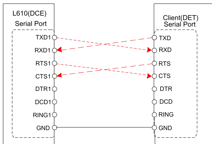
Figure 3-11 UART 4 Line connection mode
