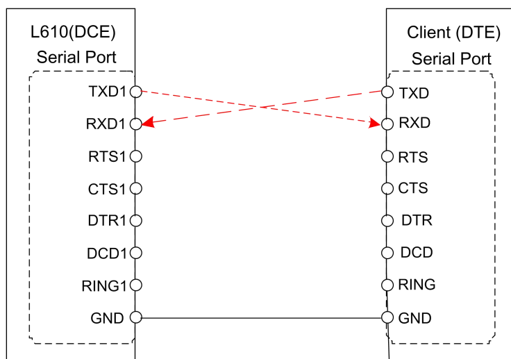
Figure 3-12 UART 2 Line connection mode
