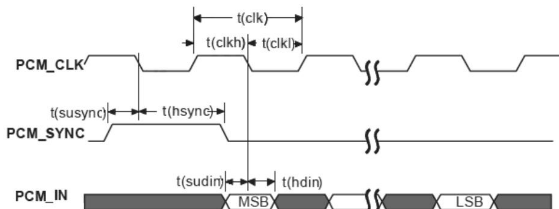
Figure 3-7 Codec to L710 module timing
