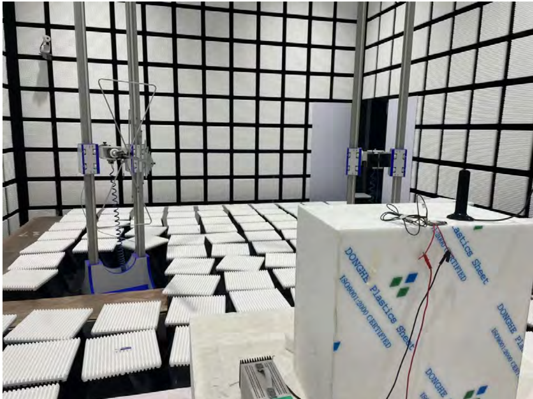
Pic2.RSE(1GHz-20GHz)
