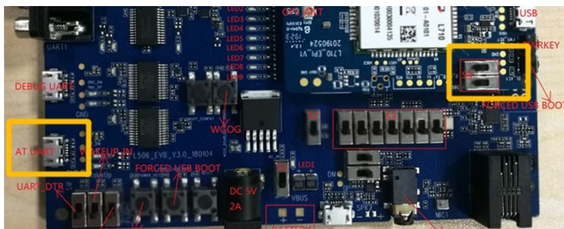
Figure5-2: USB (AT UART) Port
