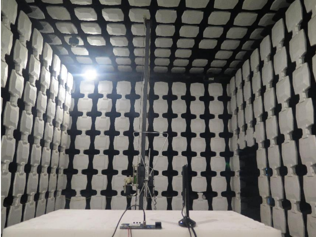
RSE (30MHz-3GHz)
