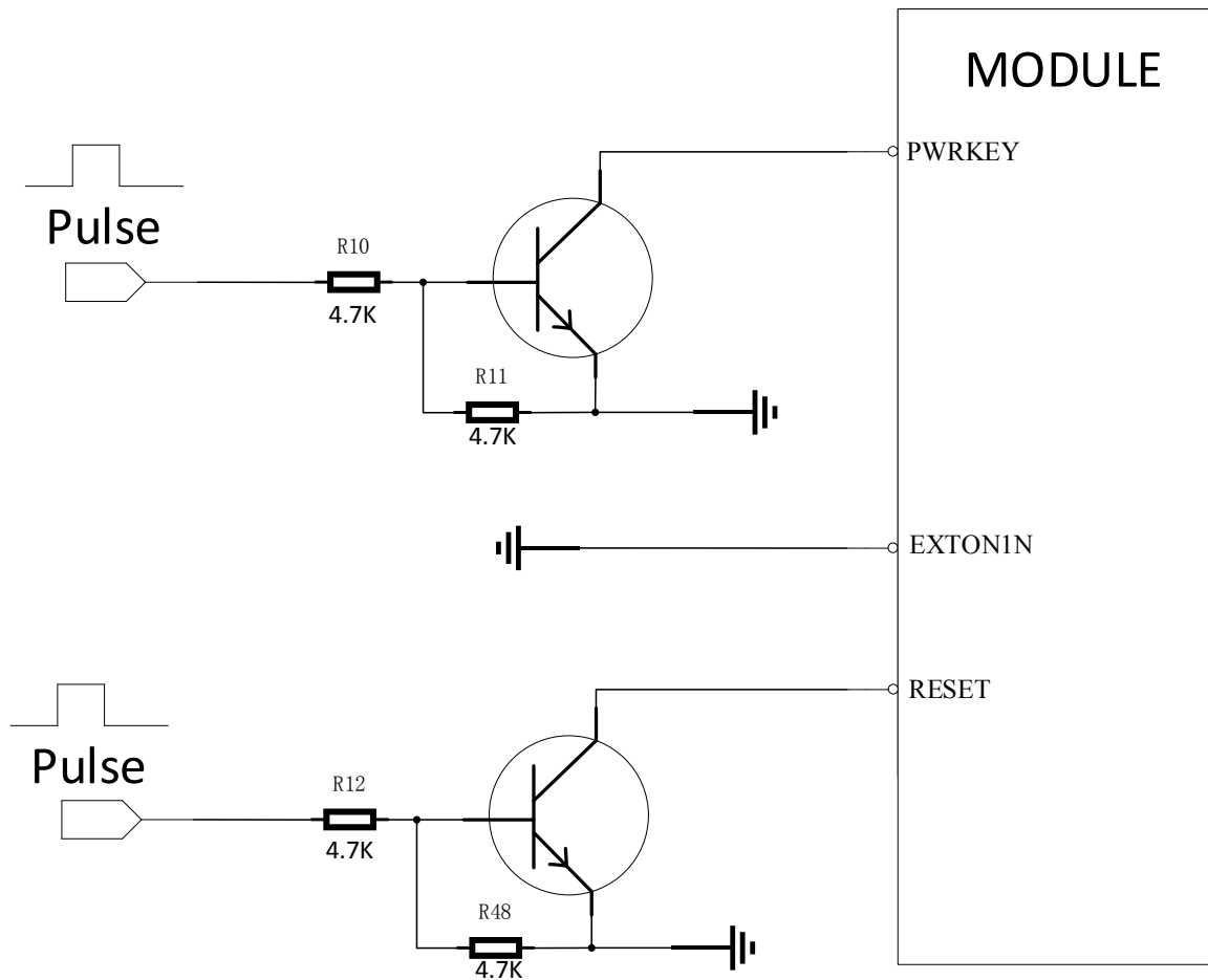
Figure 41 PWRKEY/RESET/EXT0N1N reference circuit
