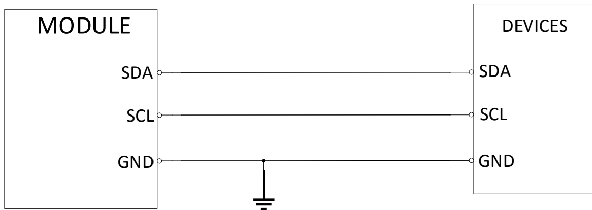
Figure 26 I2C design reference circuit
