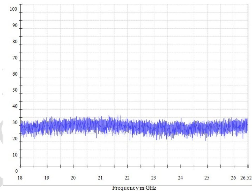
Fig.27 Radiated emission: 18 GHz - 26 GHz
