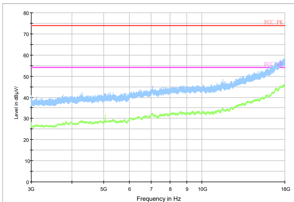
Fig.26 Radiated emission: Ch39, 3GHz-18GHz
