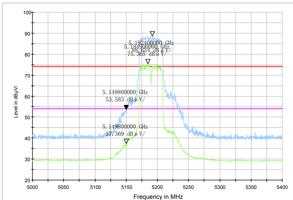
Fig 284 Frequency Band Edge: Ch38,11n 40M ANT2
