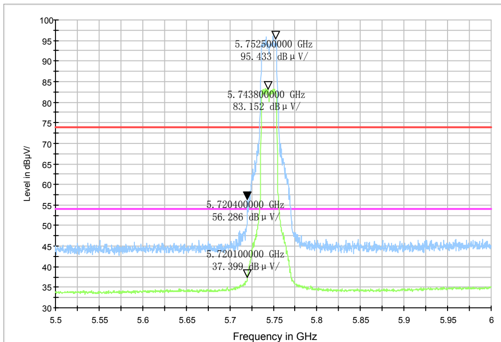
Fig 298 Frequency Band Edge: Ch149,11n 20M ANT2
