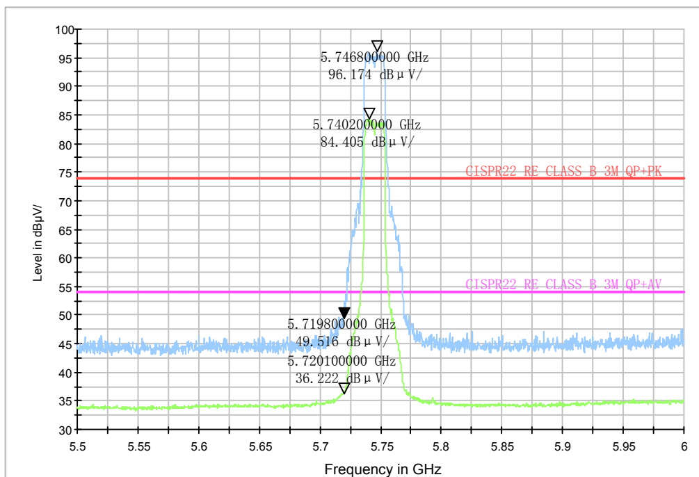
Fig. 275 Frequency Band Edge: Ch149,11a ANT2
