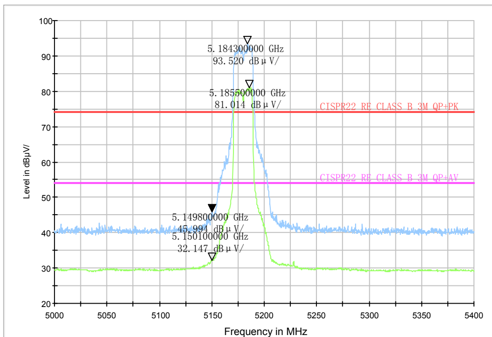
Fig 282 Frequency Band Edge: Ch36,11n 20M ANT2
