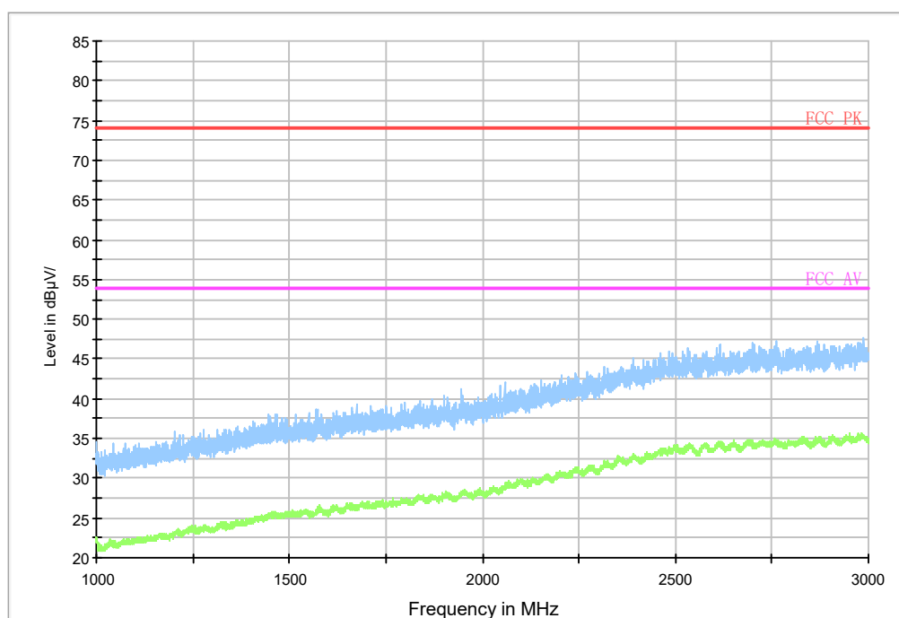
Fig. 475 Radiated emission: Ch149, 1GHz-3GHz
