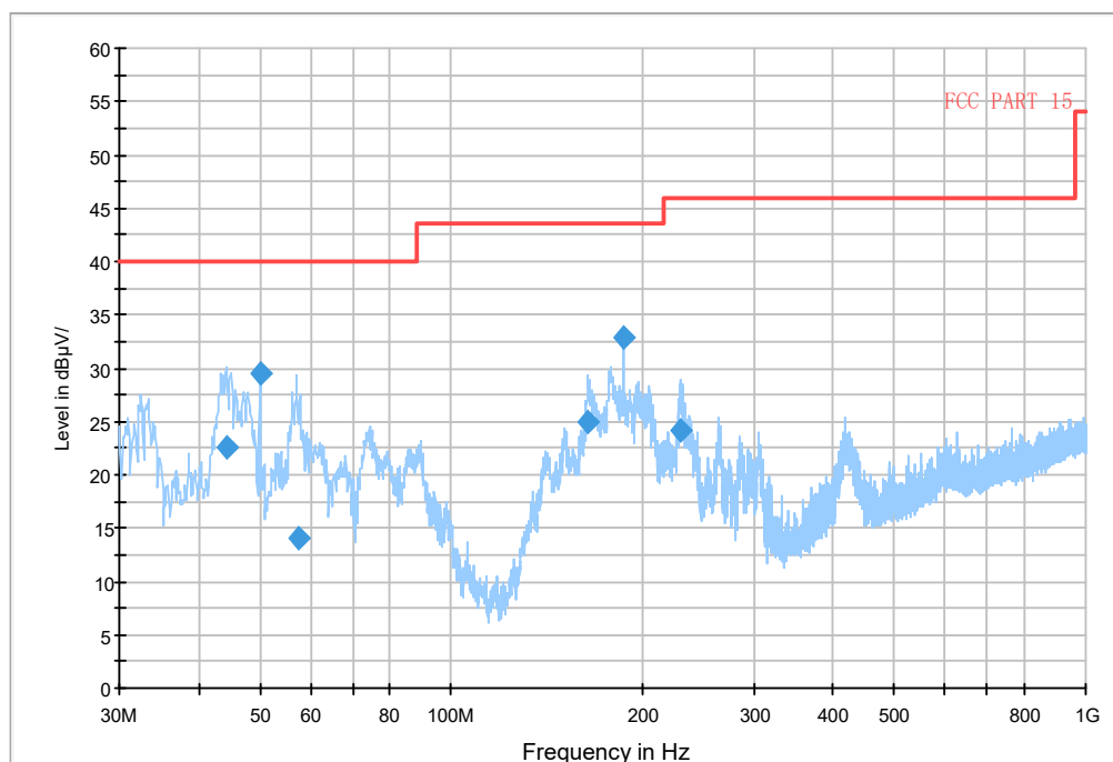
Fig. 474 Radiated emission: Ch149, 30MHz-1GHz
