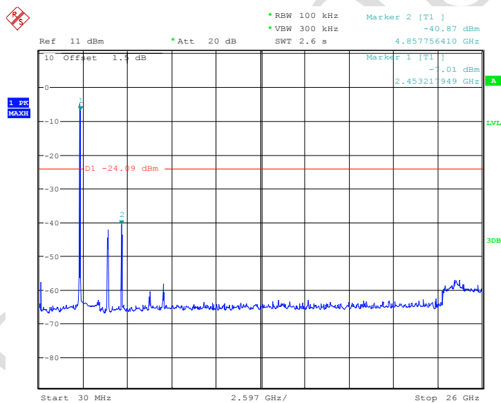
Fig.149 Conducted spurious emission: Ch6,11N40m,2437MHz(Antenna 2)
