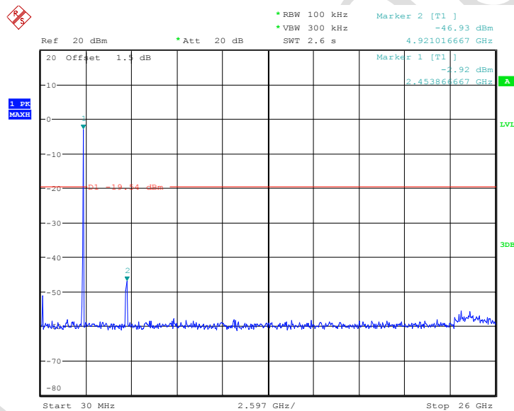
Fig.91 Conducted spurious emission: Ch11,11g,2462MHz(Antenna 1)
