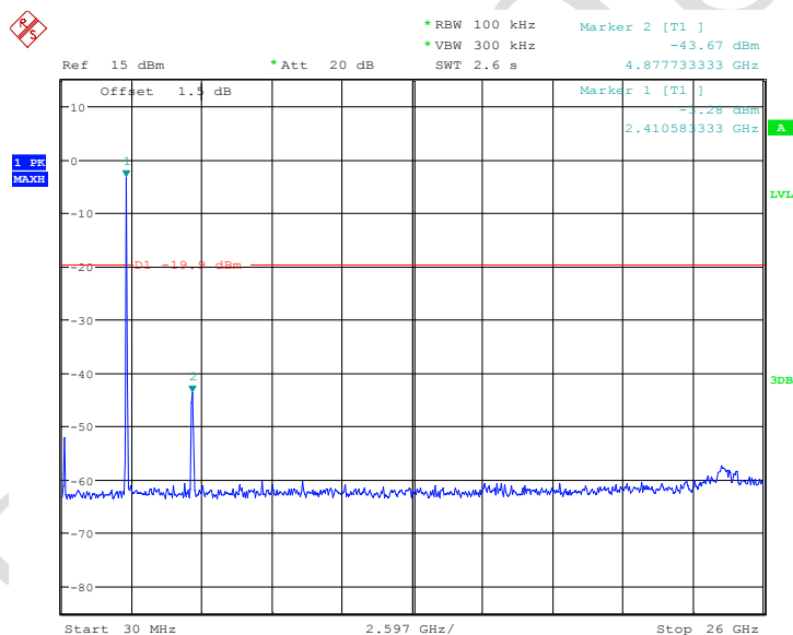
Fig.125 Conducted spurious emission: Ch6,11g,2437MHz(Antenna 2)
