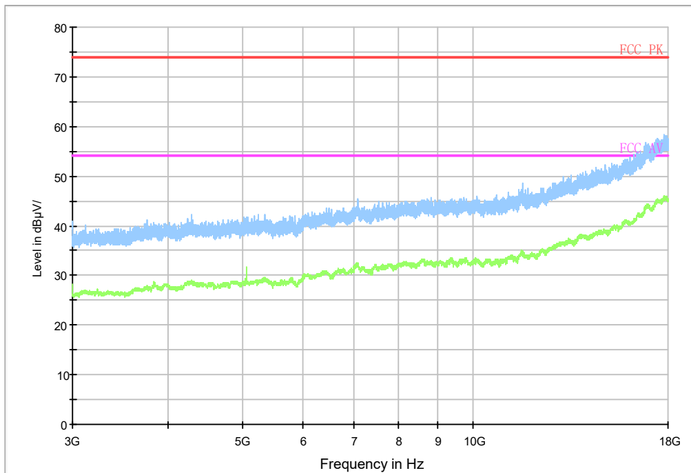
Fig.155 Radiated emission: Ch1, 3GHz-18GHz
