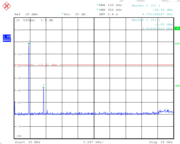
Fig.93 Conducted spurious emission: Ch1,11n,2412MHz(Antenna 1)
