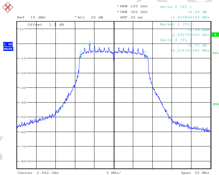
Fig.58 6dB Bandwidth: Ch11,11g(Antenna 2)
