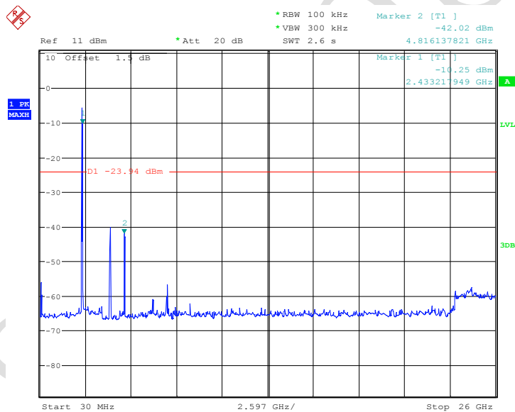
Fig.147 Conducted spurious emission: Ch1,11N40m,2412MHz(Antenna 2)
