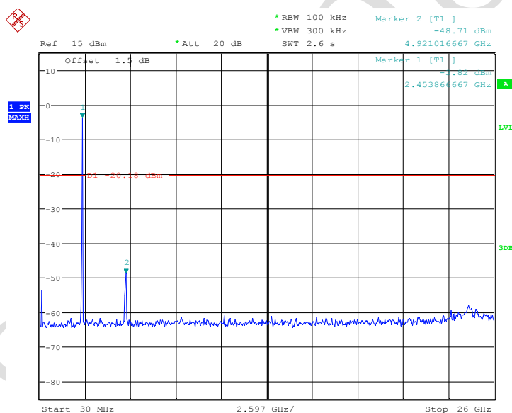
Fig.127 Conducted spurious emission: Ch11,11g,2462MHz(Antenna 2)
