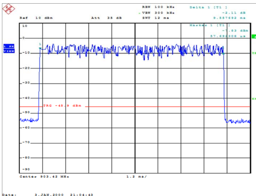
Figure 9 - Dwell Time
