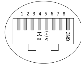
Figure 1: RJ45 Pinout
