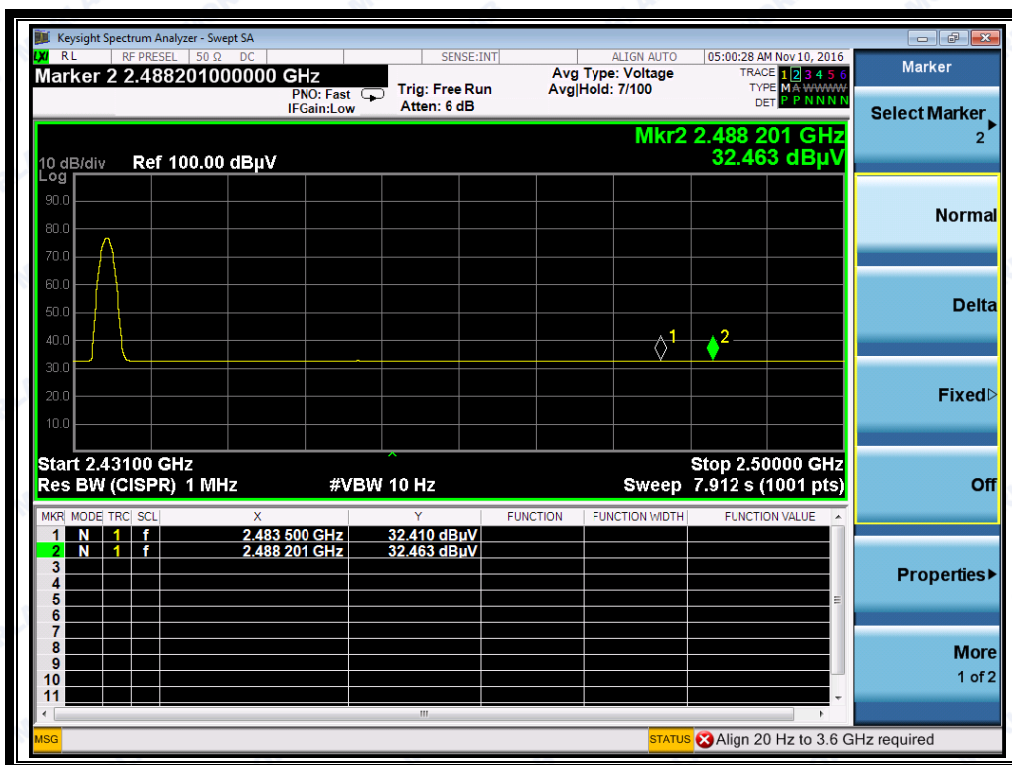
(Plot B2: Channel = 36 AVG)
