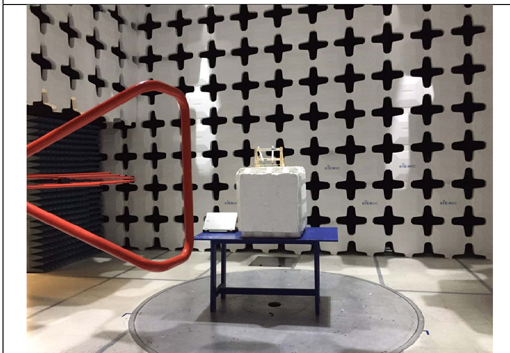
Radiated Emissions (<1GHz) – Rear View
