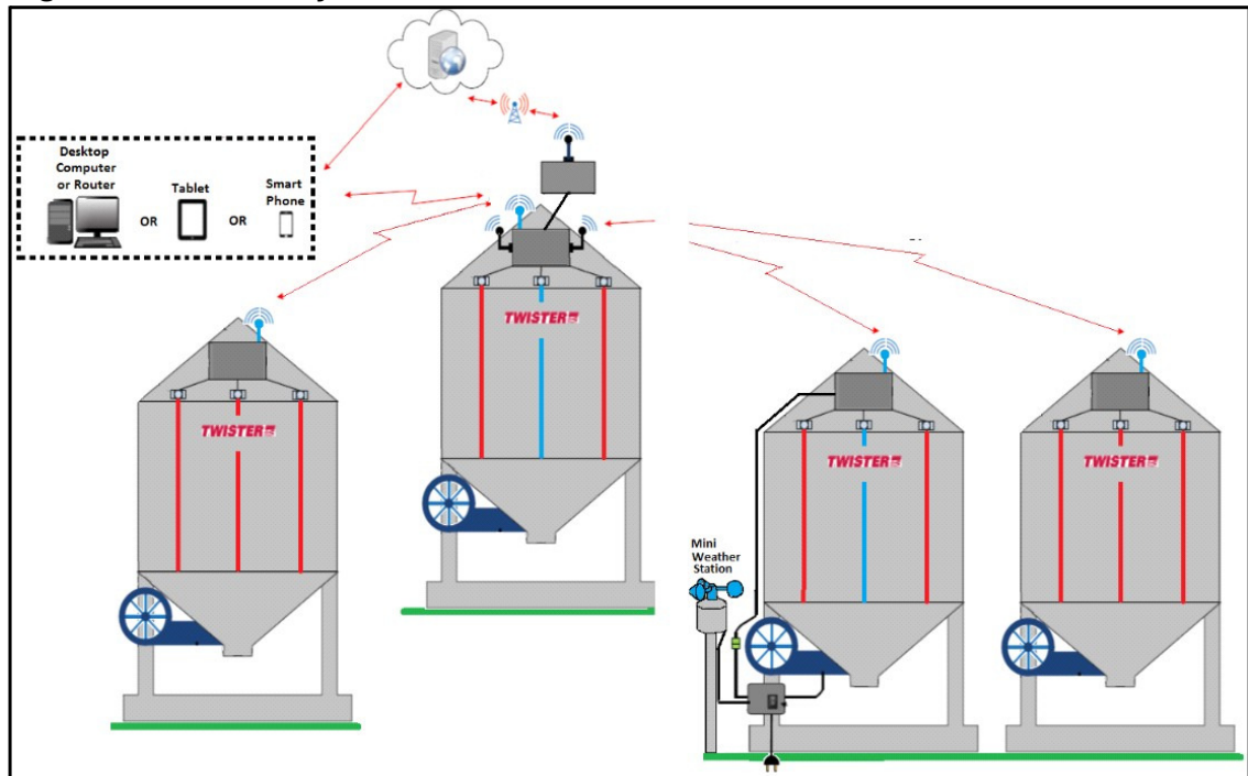
Figure 4.3 Remote System
