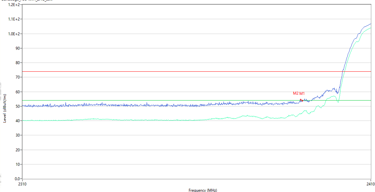
Bandedge_FCC-WIFI_2.4G_Left
