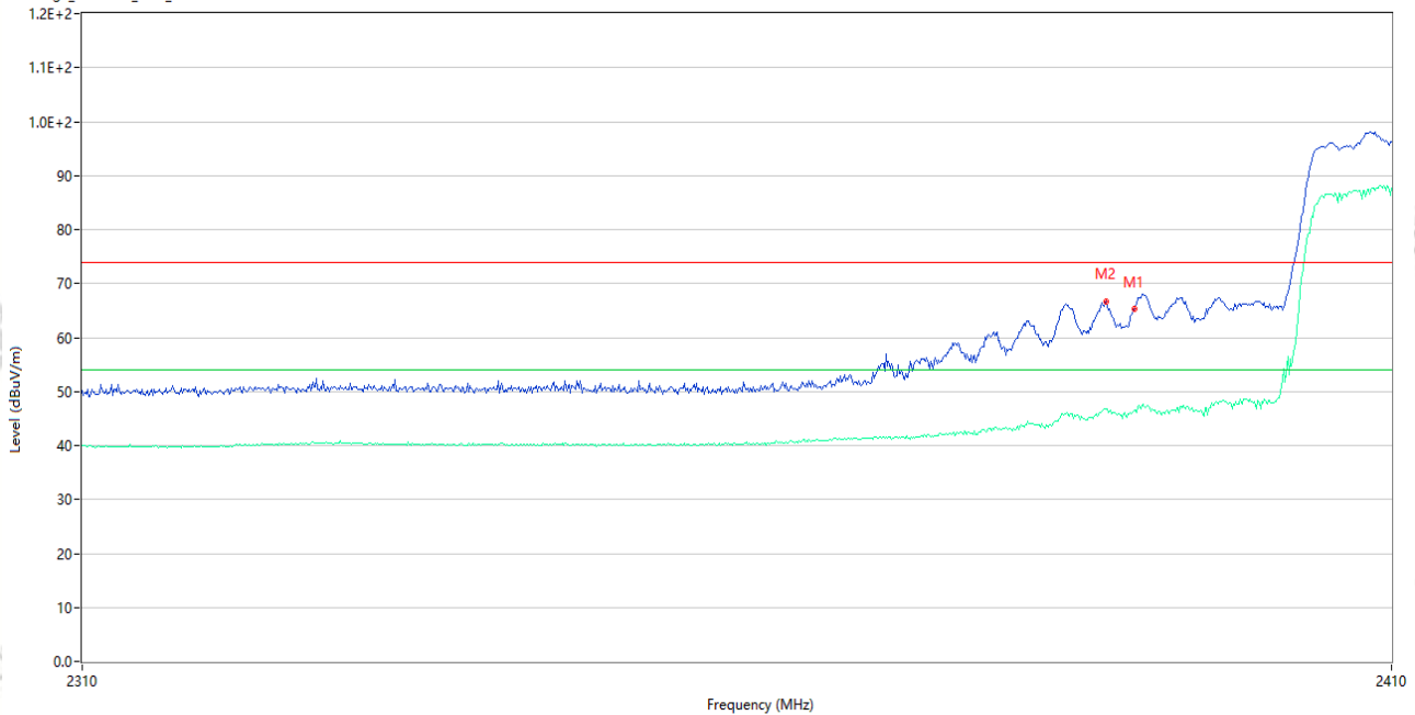
Bandedge_FCC-WIFI_2.4G_Left
