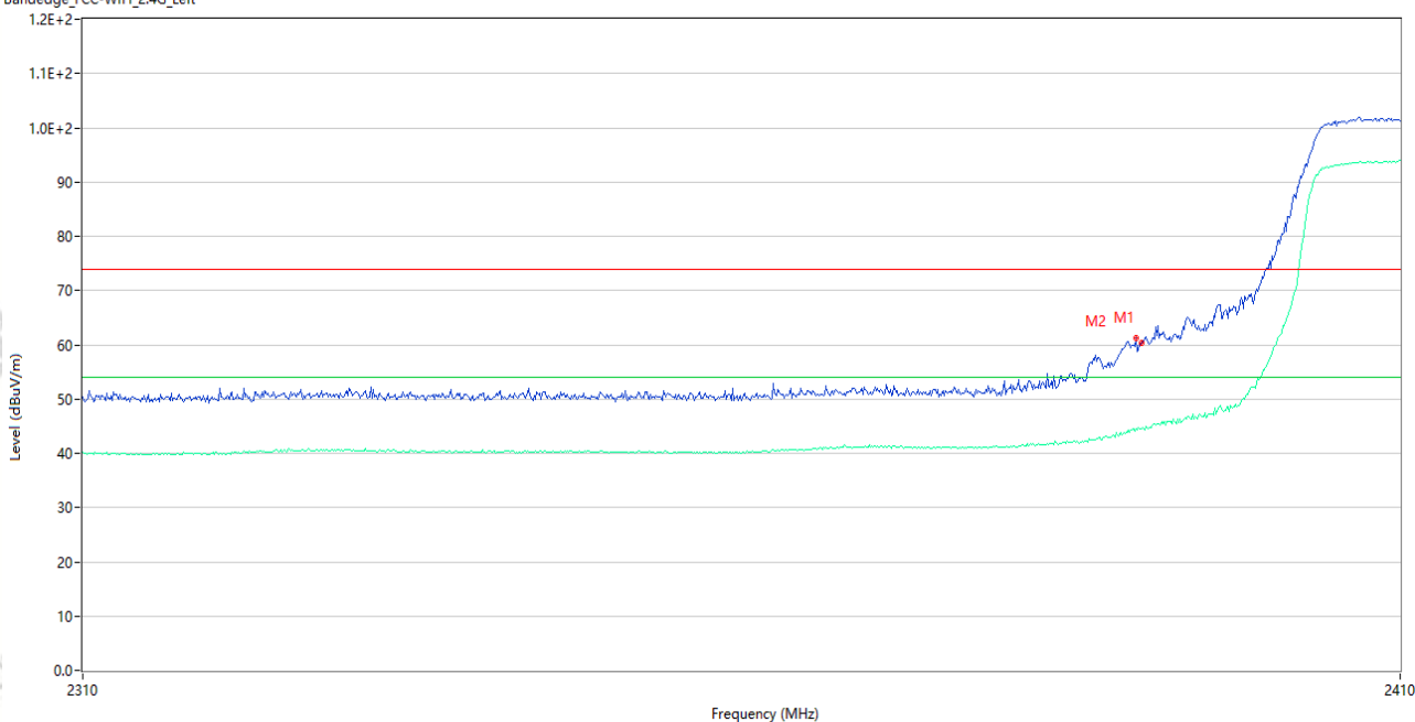
Bandedge_FCC-WIFI_2.4G_Left
