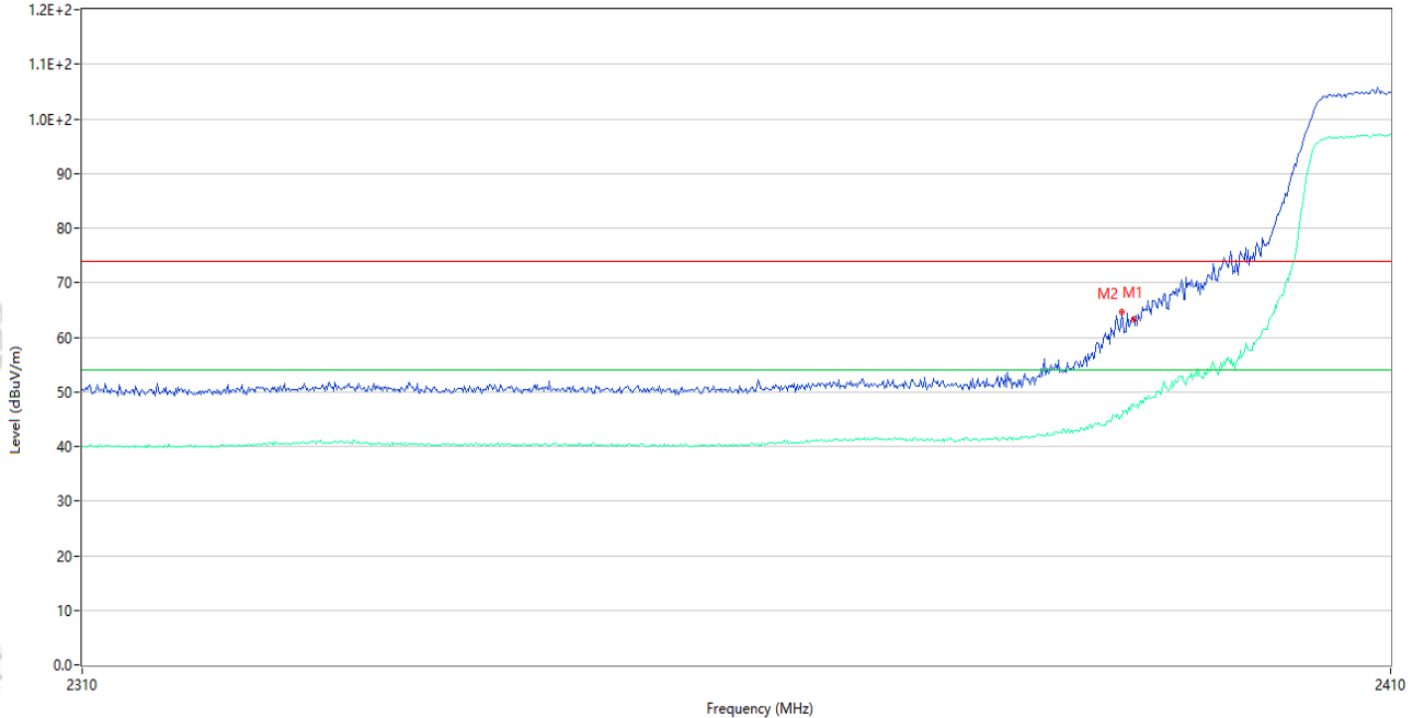
Bandedge_FCC-WIFI_2.4G_Left 1.2E+2
