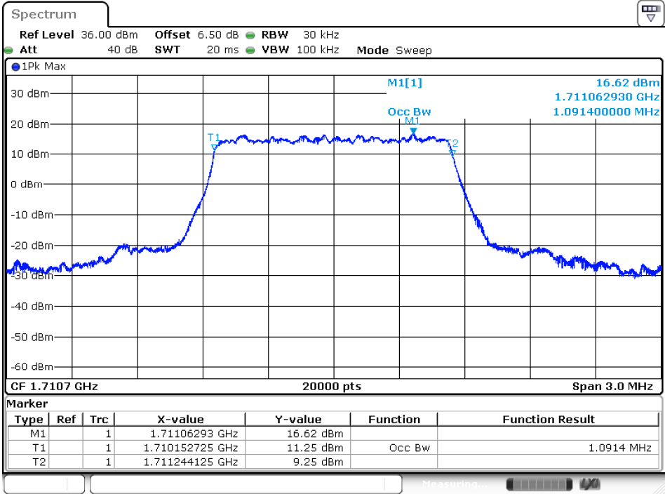
Band 66_1.4 MHz_Low_QPSK_RB6#0
