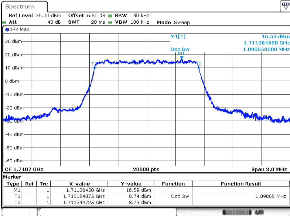
Band 66_1.4 MHz_Low_16QAM_RB6#0
