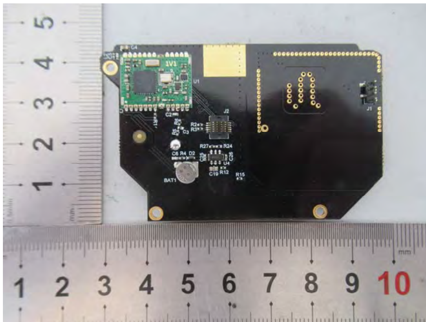
EUT – PCB-6 Top Shielding off View
