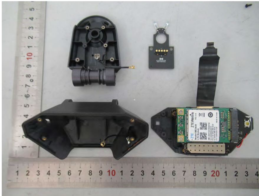
EUT – WCDMA & LTE Main Antenna View
