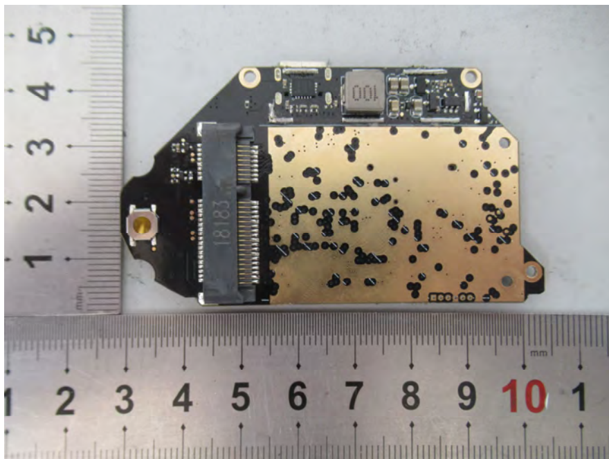
EUT – PCB-7 Bottom Shielding off View
