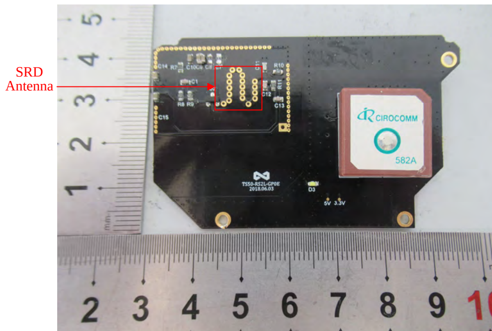
EUT – PCB-6 Bottom View
