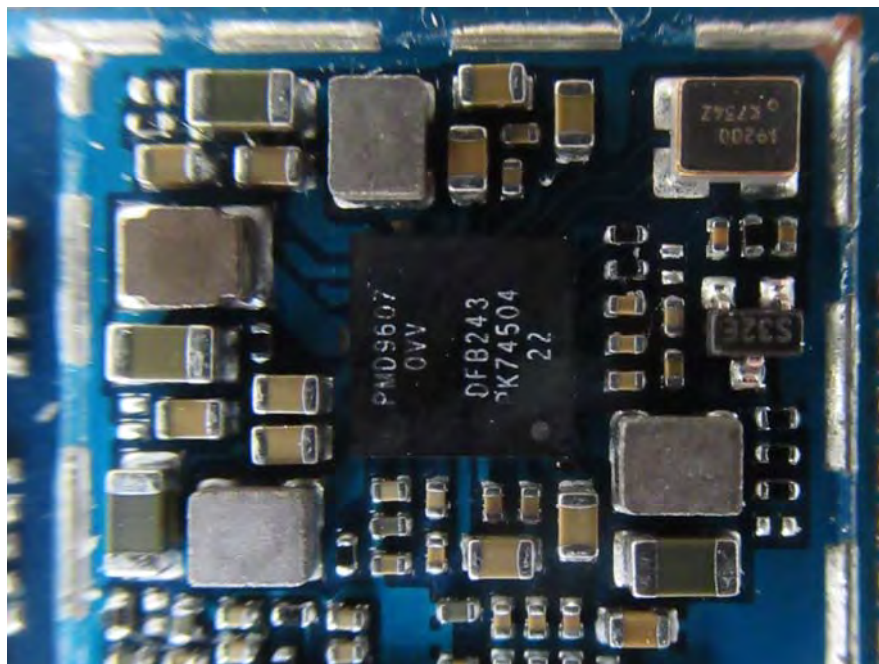
EUT – PCB-5 Top Chip View-3
