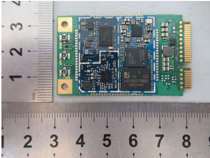
EUT – PCB-5 Top Chip View-1
