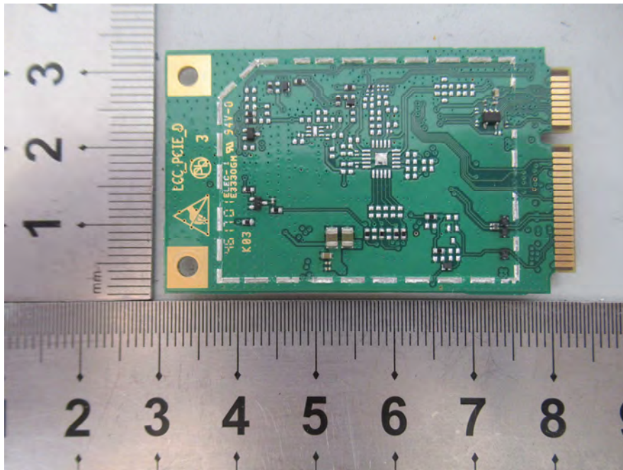
EUT – PCB-5 Bottom Shielding off View
