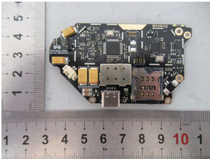
EUT – PCB-7 Top Shielding off View
