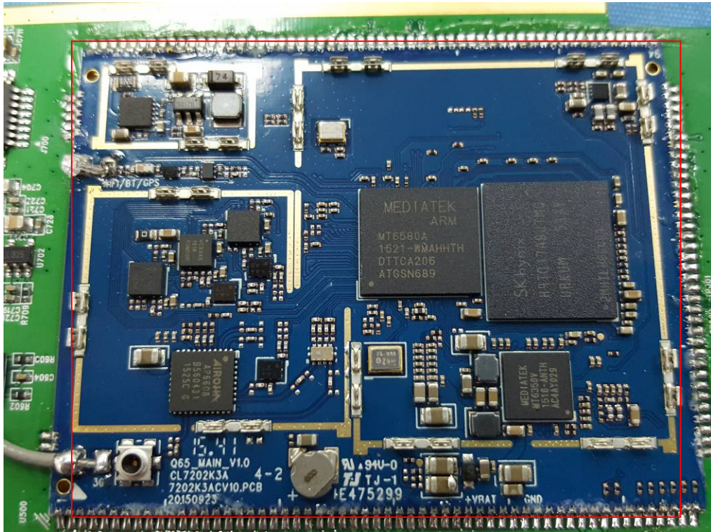
Photo 19 GSM/WCDMA/WLAN Modules
